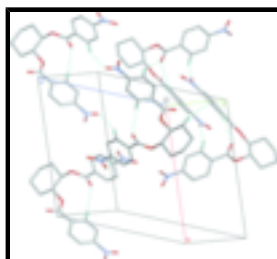
Fig. 3. The molecular packing of racemic diester with non-conventional hydrogen bonding represented as dashed lines. Hydrogen atoms not involved in hydrogen bonding have been omitted for clarity.
