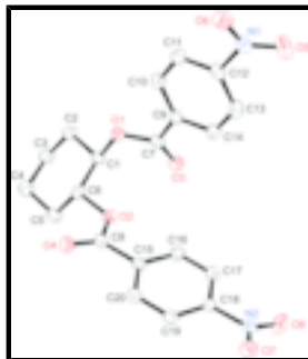
Fig. 1. The molecular structure and atom numbering scheme of (1 R *,2 R *)-diester (1 R *,6 R * in the crystallographic numbering scheme) with displacement ellipsoids drawn at the 50% probability level for non-H atoms.
